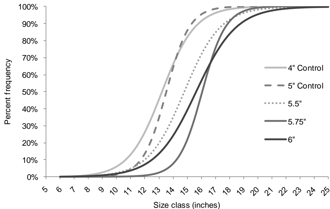
Figure 10.23 Selectivity curves of southern flounder retained in pound nets without escape panels and pound nets with different sized escape panels (NCDMF Biological Database).
